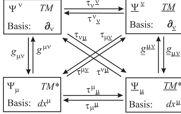
Fig. 1. Relations between the maps. The left side depicts the tangential and co-tangential spaces. The right side depicts the corresponding spaces for the anti-gravitational fields.
