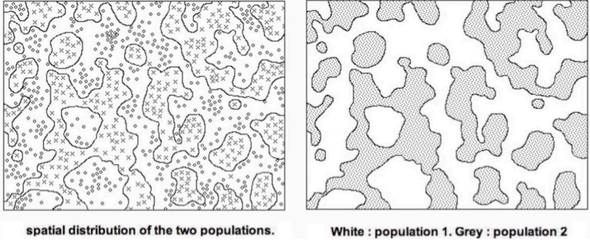
Fig.2 : Evolution of the system when |\rho^{(-)}| = \rho^{(+)}
