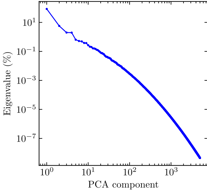
Figure 4. The spectrum of normalized eigenvalues for the first 5000 PCA components derived from a set of 30,720 GRMHD snapshots. Only 10 PCA components are necessary to reconstruct 98% of the total variance, whereas 20 can recover 99% of it.
