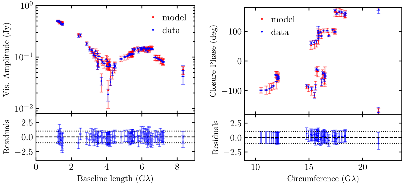
Figure 10. Left: synthetic visibility amplitude data and the amplitudes that correspond to the most likely PRIMO reconstruction. The theoretical uncertainty (see Section 3.5) is shown as error bars on the model. The residuals of the fit are shown below, with the theoretical and observational uncertainties having been added in quadrature. Right: the same but for the synthetic closure phase data.
