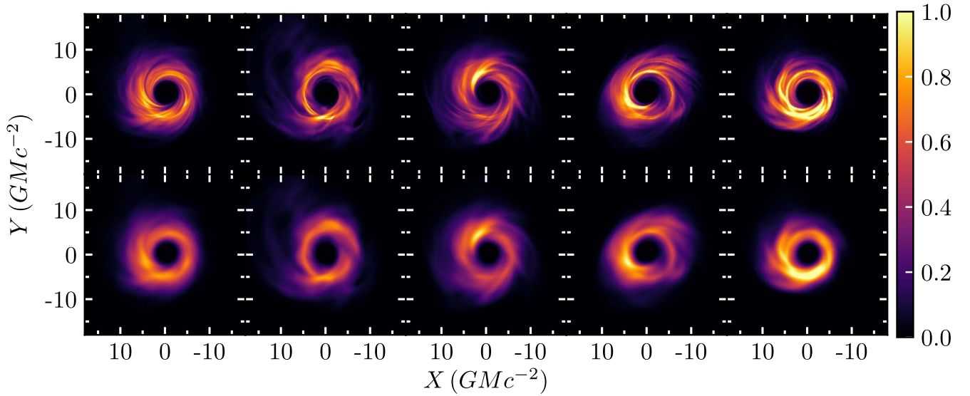
Figure 2. Top row: five representative snapshots from the MAD simulation with n_e = 5 \times 10^5 , R_{\text{high}} = 20 , i = 17^\circ , and M = 6.5 \times 10^9 M_\odot . Even within a single simulation, there is significant structural variability between the various snapshots. Bottom row: the same snapshots as the top row but filtered using a Butterworth filter with n = 2 and r = 15 \text{ G}\lambda , to mimic the finite resolution of the EHT. The brightness in each panel has been normalized such that all panels have the same total flux.
