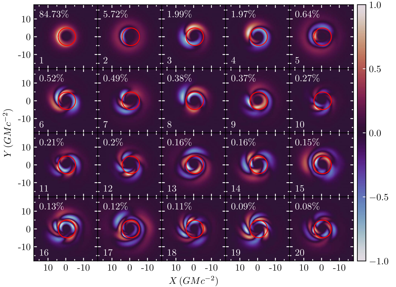
Figure 3. The first 20 PCA components for the set of simulated images employed in this paper. The respective proportions of variance explained are shown at the top left corner of each panel. Red closed curves show the analytically calculated size and shape of the black hole shadow boundary, defined as the critical impact parameter between photons that fall into the black hole and those that escape, as seen by an observer at infinity. The first PCA component is similar to the average image of the simulations, while contributions from the second component lead to thicker and thinner rings. The third and fourth components allow for either up–down or left–right asymmetries. The higher-order components describe smaller-scale structure indicative of the variance seen in the simulated snapshots. Each panel is normalized such that the full range of values falls within the range of the color bar.
