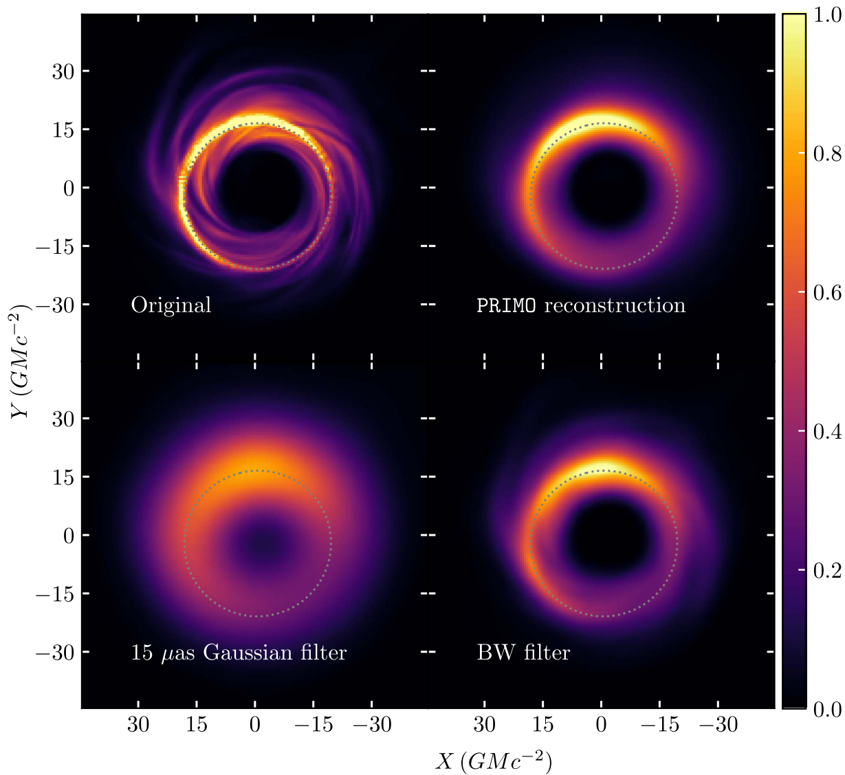
Figure 9. Top left: simulated image used for the generation of the first synthetic data set. Top right: the highest likelihood PRIMO reconstruction for the synthetic data. PRIMO can accurately reproduce the depth and shape of the brightness depression, the size and width of the ring of emission, and the brightness asymmetry of the ring. Bottom left: the original image blurred by a Gaussian filter with a width of 15 \mu\text{as} , which mimics the nominal resolution of the EHT (see text). Bottom right: the simulated image convolved with a Butterworth filter with radius r = 15 \text{ G}\lambda and index n = 2 . The brightness in all panels has been normalized such that all images have the same total flux, with the exception of the Gaussian-broadened image, which has a total flux that is 1.5 times higher than the other panels. In all panels, the gray dotted circles indicate the analytically calculated size and shape of the black hole shadow. The original and filtered images have been rotated to the position angle used to generate the synthetic data set and the PRIMO reconstruction has been rotated by the position angle \phi derived from the model.
