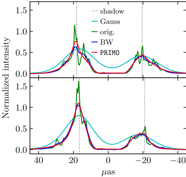
Figure 11. Comparison of the horizontal (top) and vertical (bottom) cross sections of the images shown in Figure 9. The curves show the original snapshot (green), the snapshot filtered with a Butterworth filter (blue), the most likely PRIMO reconstruction (red), the snapshot filtered with a 15 \mu\text{as} Gaussian (cyan), and the analytically calculated edges of the black hole shadow (gray dotted vertical lines). The cross sections are normalized such that all images have the same total flux, except for the Gaussian-broadened image, which has 1.5 times the flux of the other images. The y-axis is in arbitrary units. PRIMO can accurately reproduce the main features of the image and does not introduce a significant bias in the ring size.
