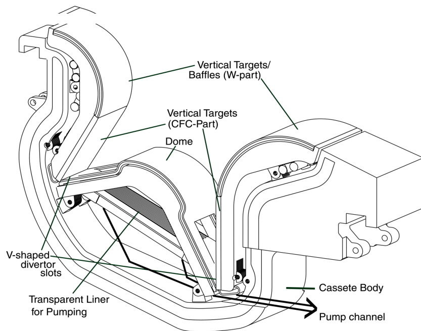
Figure 4.2-2 Divertor Cassette
