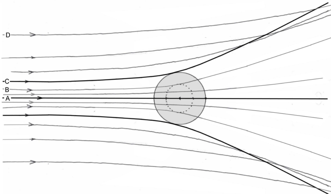
Figure 2: Deviation of positive-energy photons by a negative mass.
